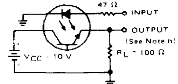
TEST CIRCUIT A PHOTOTRANSISTOR OPERATION
