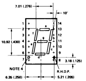
F,G FRONT VIEW
