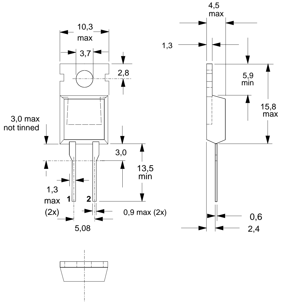
Fig. 10. TO220AC; pin 1 connected to mounting base.
