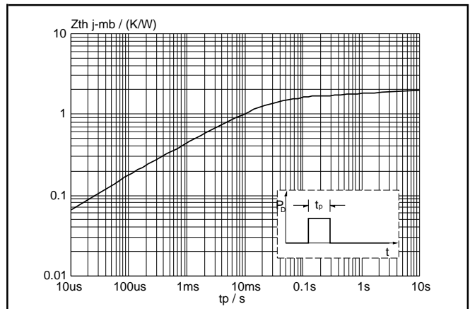
Fig.9. Transient thermal impedance Z_{th} = f(t_p)
