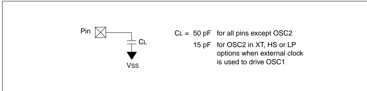
FIGURE 13-1: LOAD CONDITIONS
