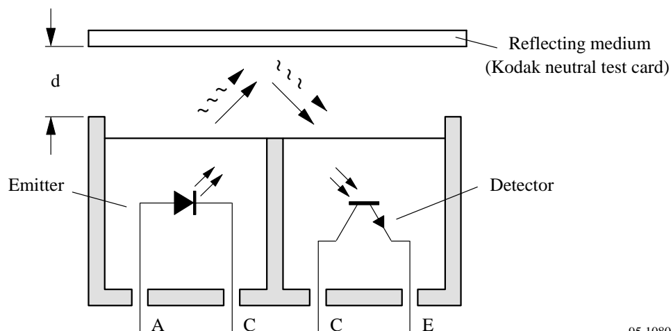
Figure 1. Test circuit
