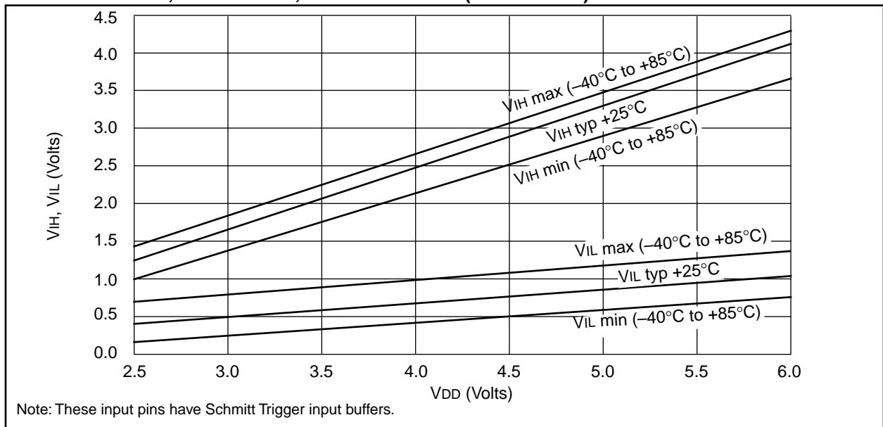
FIGURE 20-9: V_{IH} , V_{IL} OF \overline{MCLR} , T0CKI AND OSC1 (IN RC MODE) vs. V_{DD}
