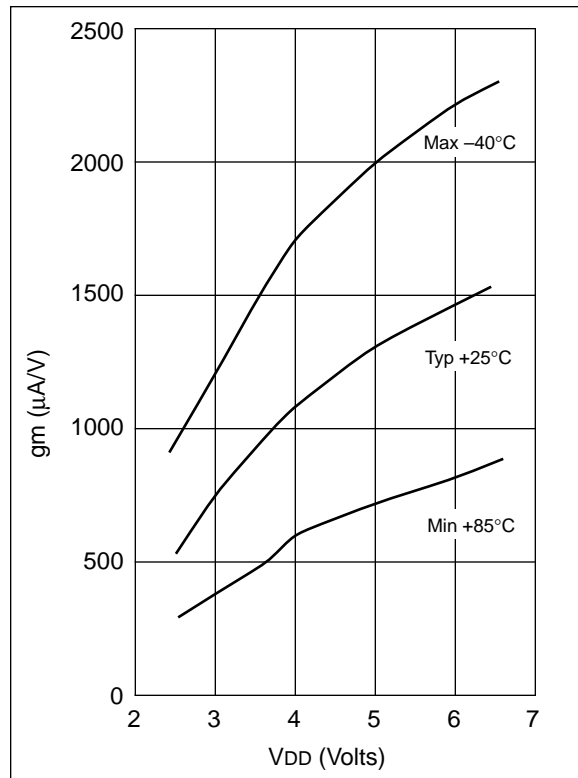
FIGURE 18-19: TRANSCONDUCTANCE (gm) OF XT OSCILLATOR vs. VDD
