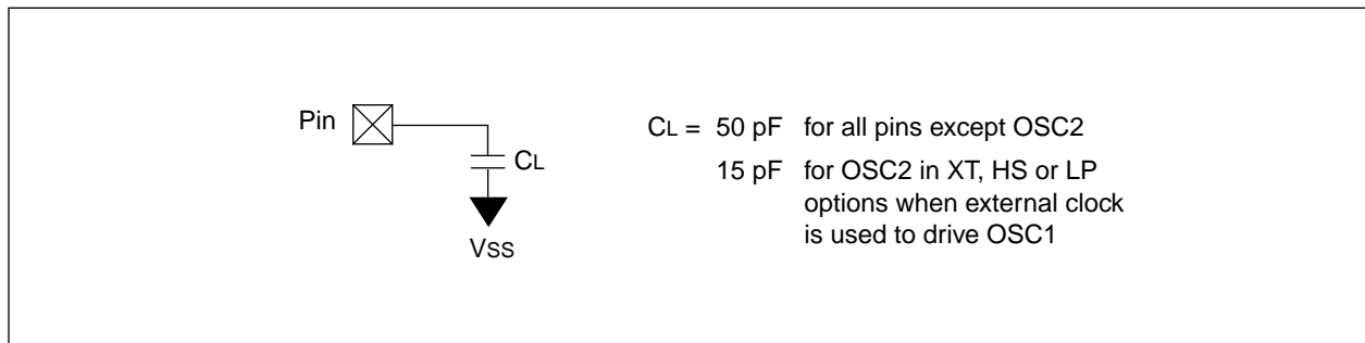
FIGURE 19-1: LOAD CONDITIONS - PIC16C54B/CR54B/C56A/CR56A/C58B/CR58B, PIC16CR5X
