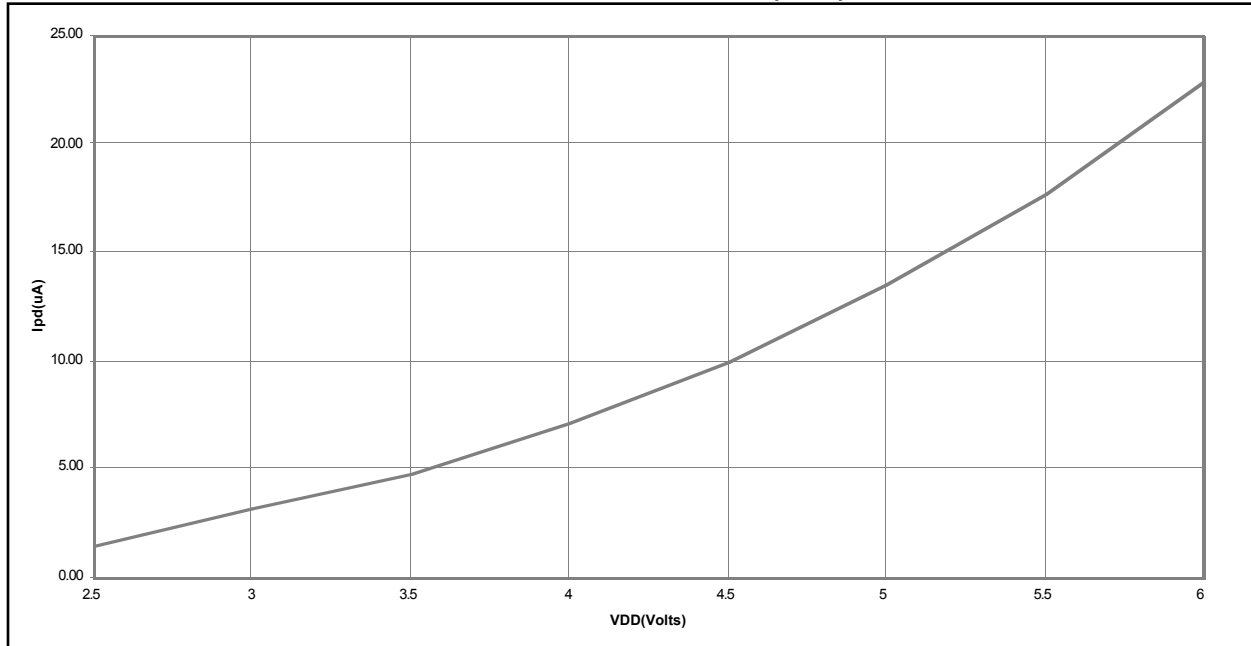
FIGURE 18-6: TYPICAL I PD vs. V DD , WATCHDOG ENABLED (25°C)
