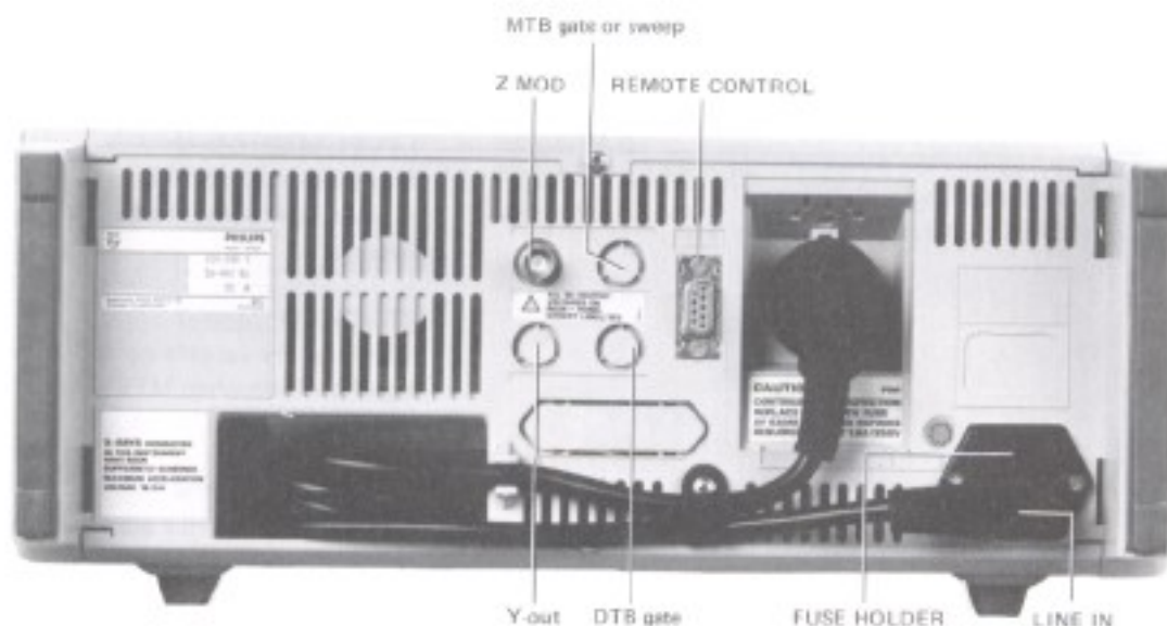
Figure 3.4 Rear view of the oscilloscope.
