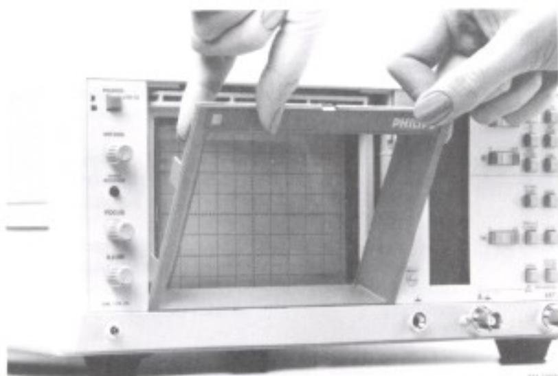
Figure 4.1 Removing the bezel and the contrast filter.
