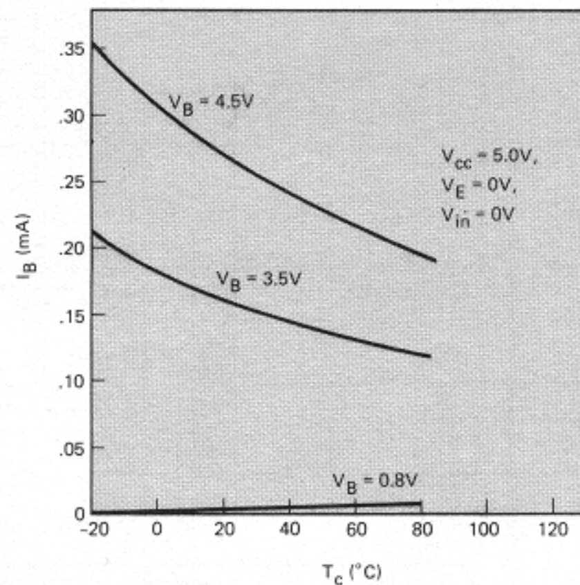
Figure 6. Typical Blanking Control Input Current Vs. Temperature, 5082-7340.
