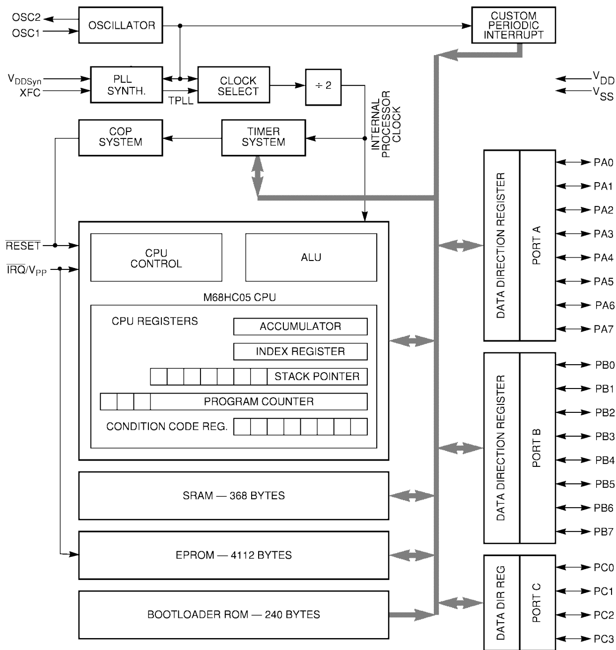
Figure 1-1: Block Diagram
